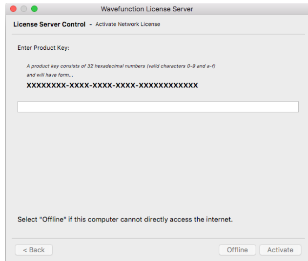
Macintosh version
