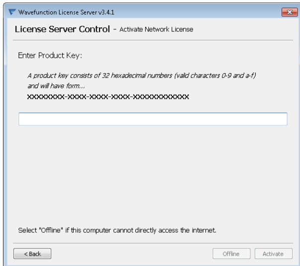
Windows version
