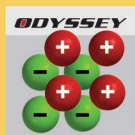
Ionic Bonding
