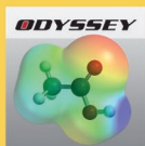
Functional Groups
