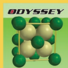
Ionic Solids
