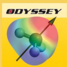
Polar Bonds and Molecules
